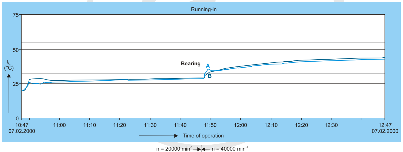
Diagram 4: Running-in n \cdot d_m = 1.6 million ( \text{min}^{-1} \cdot \text{mm} )
