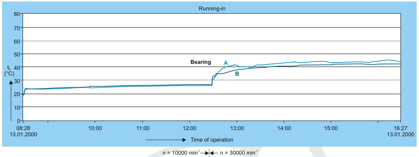
Diagram 3: Running-in n \cdot d_m = 1.3 million ( \text{min}^{-1} \cdot \text{mm} )
