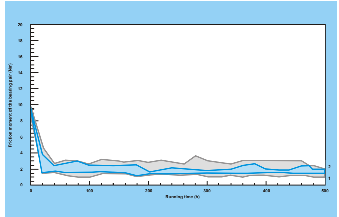
Diagram 1: FE8 test run with tapered roller bearing 536048 ( \cong 31312); axial load F_a = 10 \text{ kN} ; speed n = 3000 \text{ min}^{-1} ; time of operation 500 h Lubrication with TURMOGREASE® Li 802 EP
